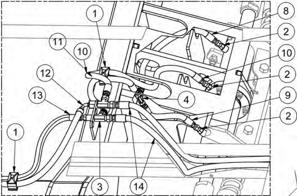
DETAIL A
